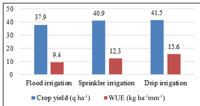
Effect of different irrigation systems on grain yield and WUE of wheat crop
