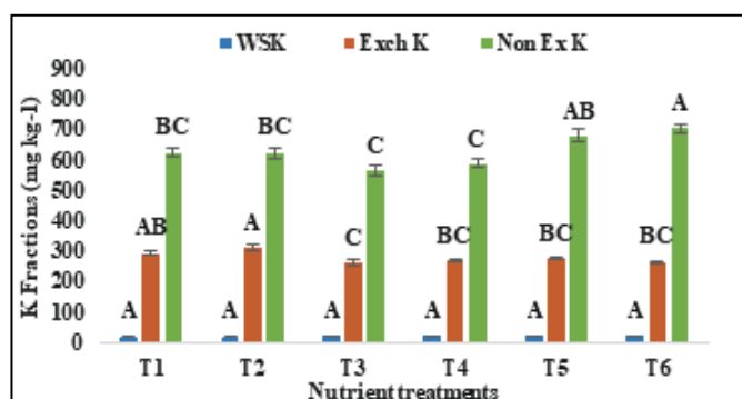
Long term nutrient management effect on soil potassium (K) fractions (mg kg -1 )
