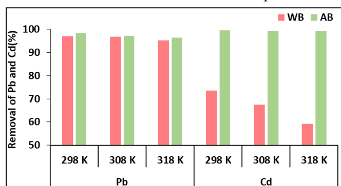
Removal of Pb and Cd at different temperature
