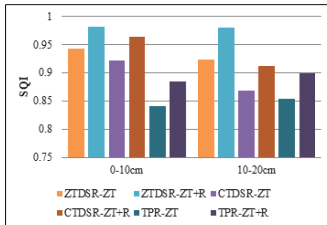
Effect of different tillage and crop establishment techniques on SQI. (ZT- Zero Till, DSR- Direct seeded Rice, TPR- Transplanted Rice, R-Residue)
